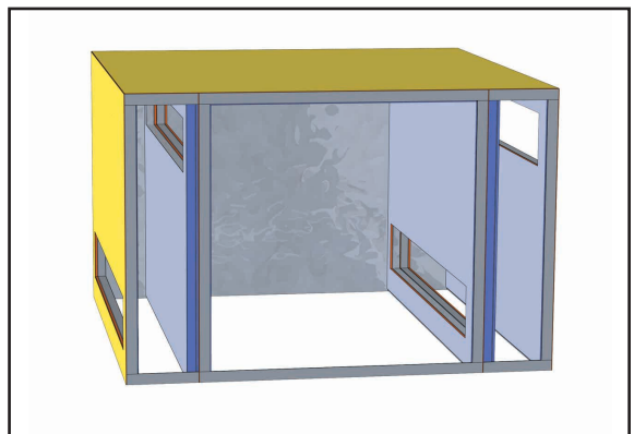
Typical enclosure construction showing air inlet/outlet.
