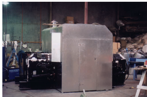
Existing enclosures can be improved substantially using MultiGrade's absorption and barrier construction. With up to 45% perceived improvement over the use of plain foam.
